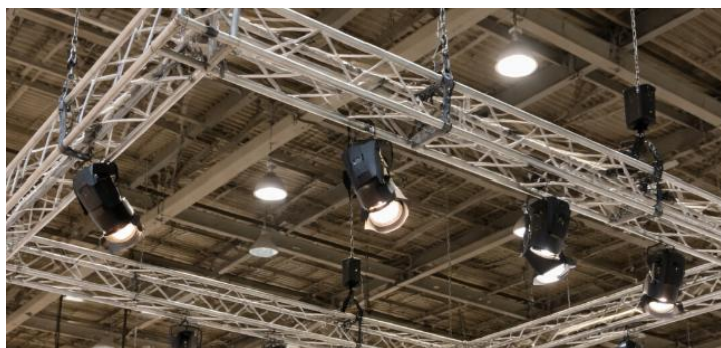
Lighting truss structures in various sizes and configurations for stand illumination.
